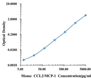
Mouse CCL2/MCP-1 Typical Standard
